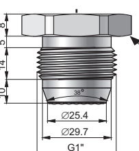
CG1-S38 type G1" with flush diaphragm
