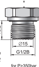
CG1/2 type G1/2" with flush diaphragm
