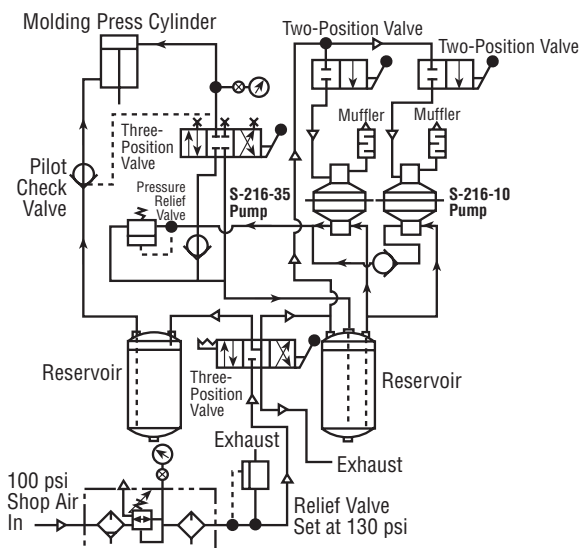
HIGH-LOW PUMP SYSTEM FOR MOLDING PRESS
