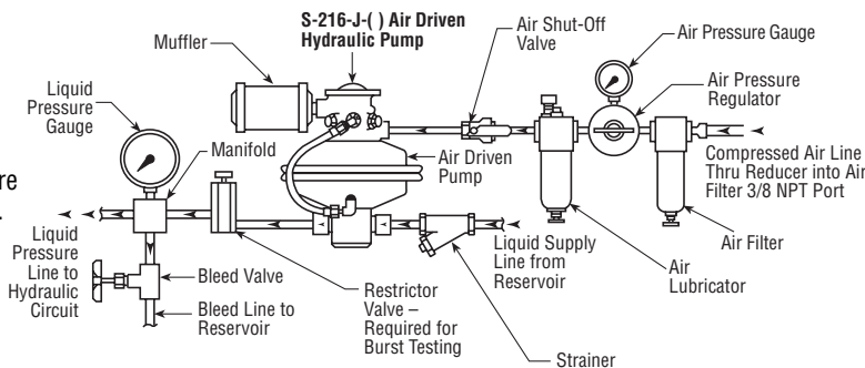
PUMP AND ACCESSORIES — TYPICAL ARRANGEMENT
